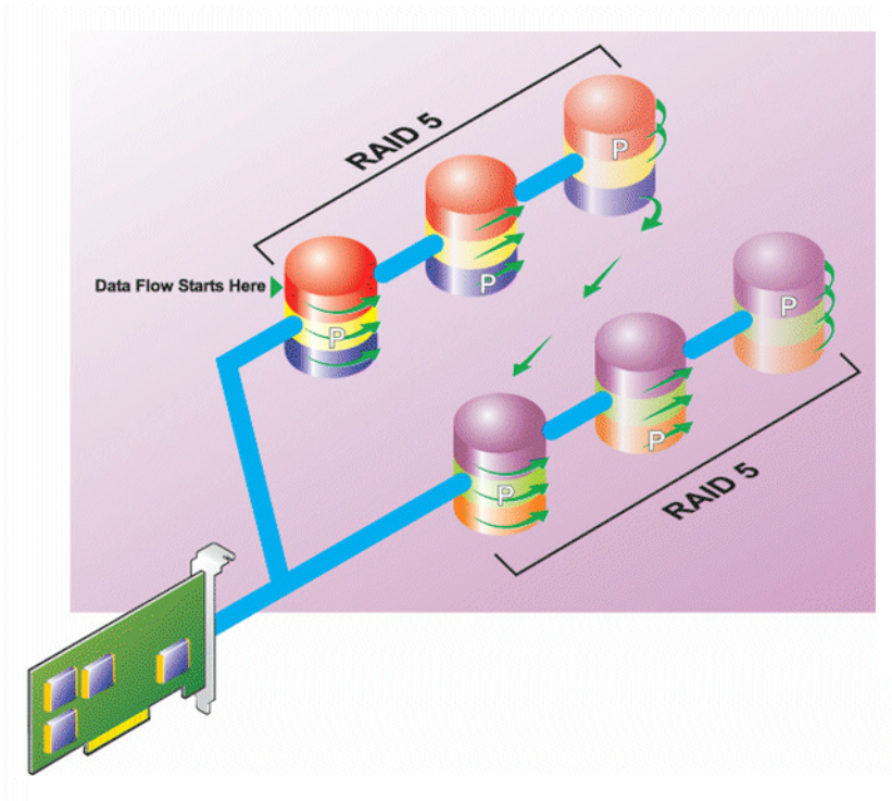
Figure 3-6. RAID 50
