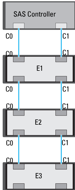
Figure 8-1. Daisy Chain Configuration
