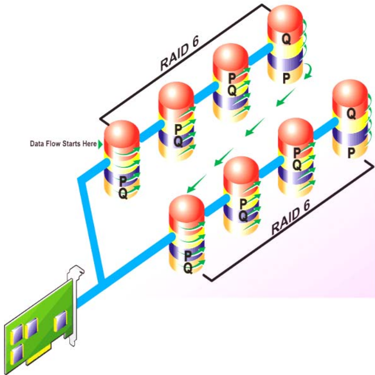
Figure 3-7. RAID 60
